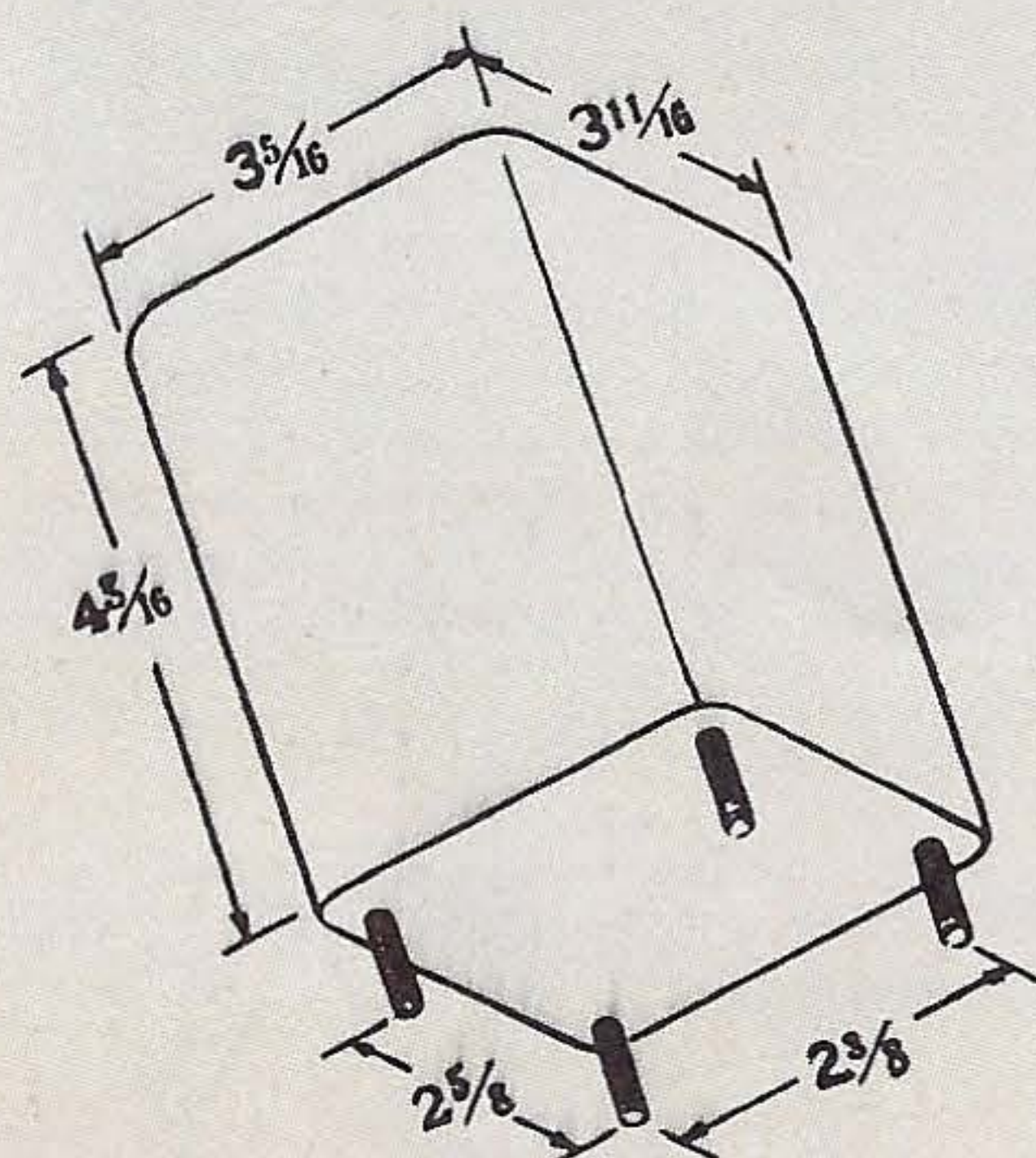
B-TYPE MOUNTING (Driver Transformer No. BD-1)
