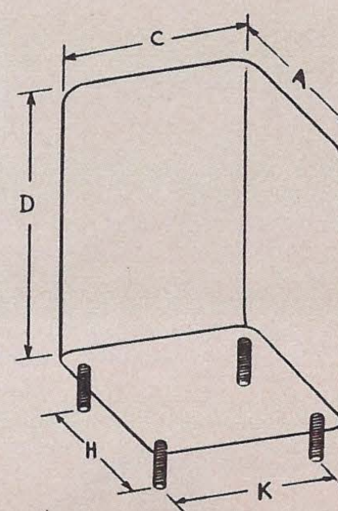
B-TYPE DIMENSIONS
