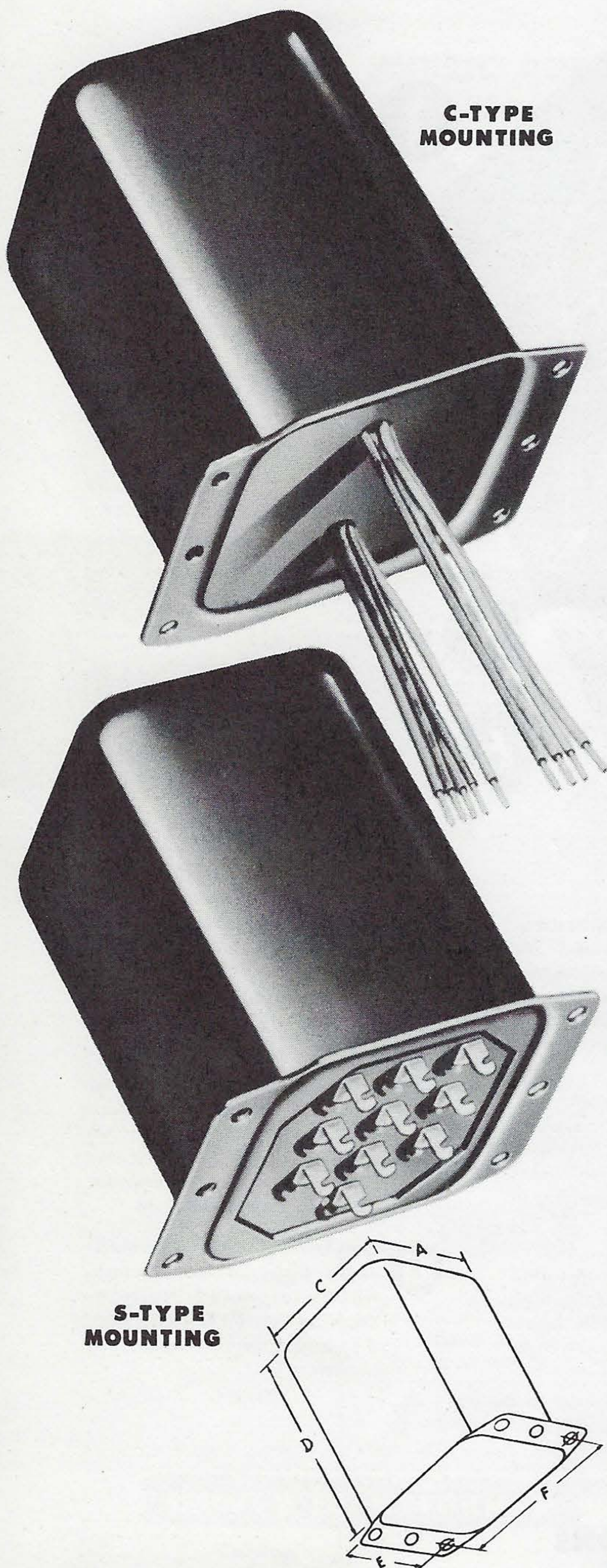
C-AND S-TYPE DIMENSIONS
