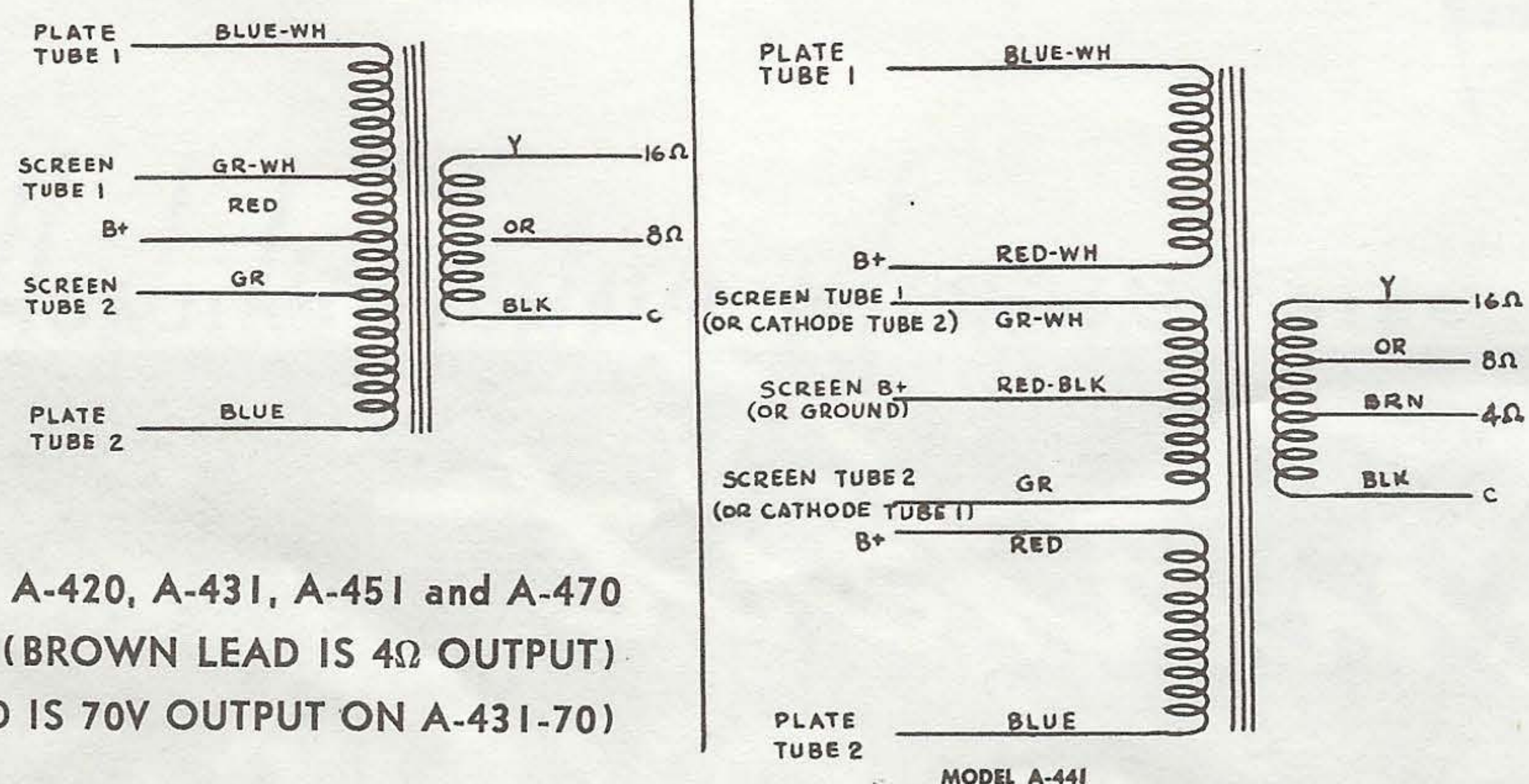
OUTPUT TRANSFORMER COLOR CODING
