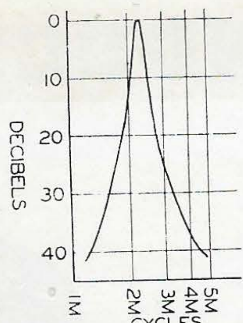
TYPICAL BPI CURVE
