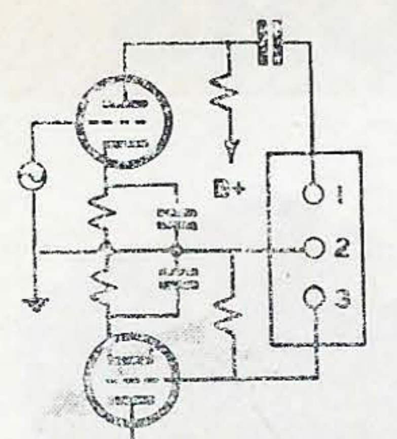
INTERSTAGE FILTER CONNECTIONS
